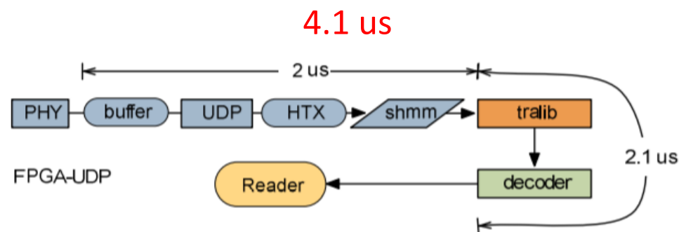
Figure 10. Latency with Kernel Bypass
