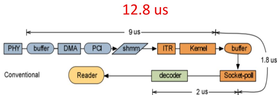
Figure 9. Latency of a the Baseline System
